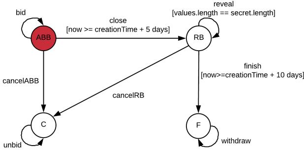
Fig. 2. Blind auction example as an ASM.
