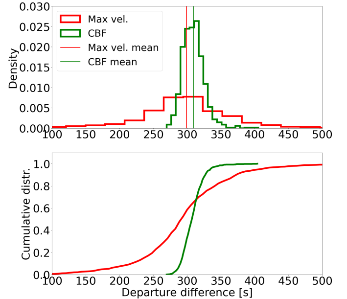
Fig. 2: Distributions of departure differences for all stops are shown. Top: departure differences in the CBF controlled case are shown in green, and the max velocity case in red. Bottom: The cumulative distribution of departure differences are shown.
