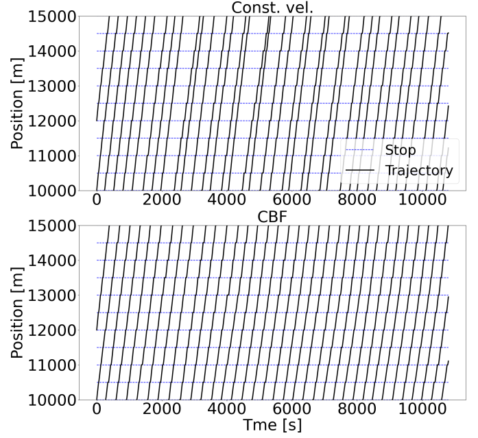
Fig. 1: Space-time trajectories for vehicles are shown (black) along the network with stops (blue). Top: trajectories of vehicles controlled by the max-velocity controller are shown. Bottom: trajectories of vehicles controlled by the CBF are shown.
