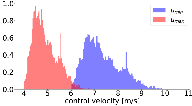
Fig. 4: The distributions of minimum and maximum allowed speeds by the CBF are shown for experiment 1.
