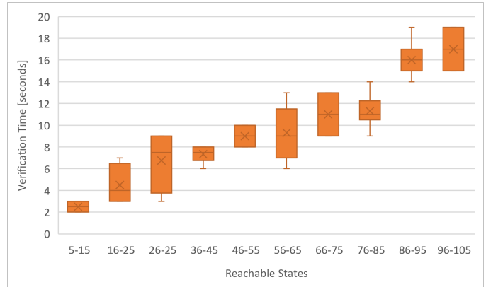
Fig. 22. Verification time and the number of reachable states for various contracts.
