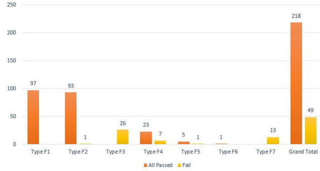
Fig. 14. Verification results for ERC20 tokens.
