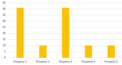
Fig. 20. Verification results ERC20 tokens by Properties
